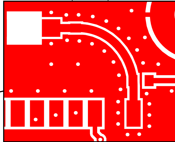
DETAIL RF Trace (Scale 8:1)
